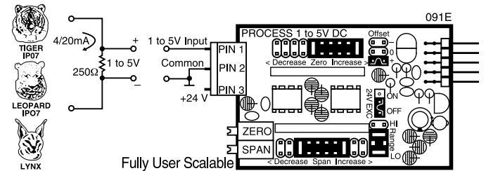
IP07: Universal Process Input 2V/5V/10V/20V/200V/2mA/20mA/Custom
